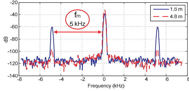
Figure 9. Measurement of the spectrum at 2.45 GHz (at 1.6 m solid line and 4.8 m dotted line).
