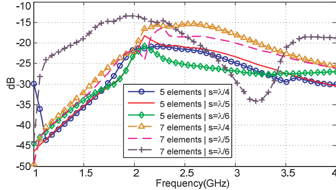
Figure 5. Return loss of a circular corrugated horn.
