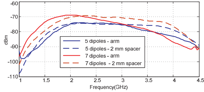
Figure 10. Comparison of FSS structure directly on contact with the arm and separated with a spacer of 2 mm [18].
