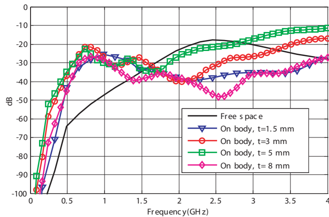
Figure 8. Simulated differential RCS of an FSS with 5 elements in free space and on body for different thicknesses of the fat layer ( t ).
