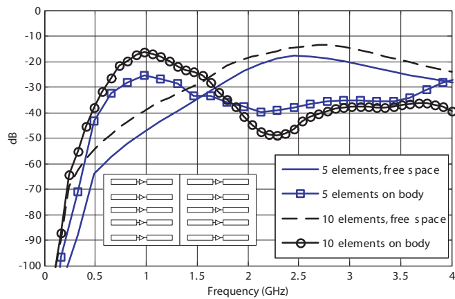
Figure 7. Simulated differential RCS of an FSS with 5 elements and 10 elements (distributed in two rows, see inset figure) in free space and on body.
