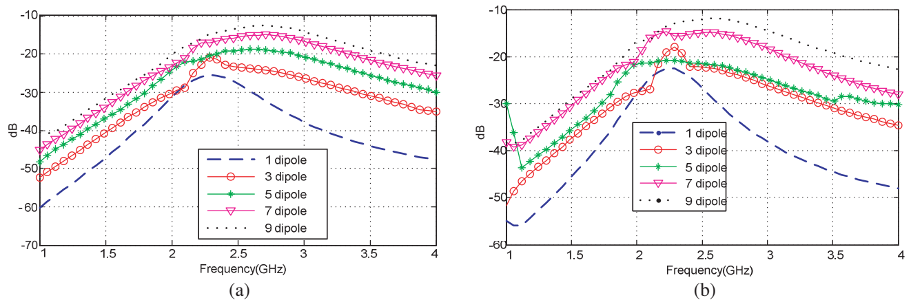
Figure 4. Comparison of FSS structure with different numbers of elements (a) in free space and (b) printer over a thin substrate.
