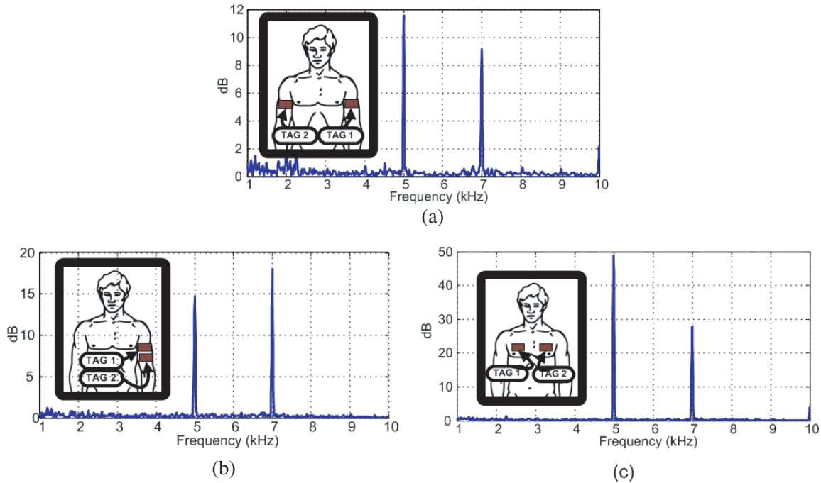
Figure 11. Received level at baseband after the A/D on the reader for two tags modulated at 5 kHz (Tag 1) and 7 kHz (Tag 2), respectively, at different body locations.
