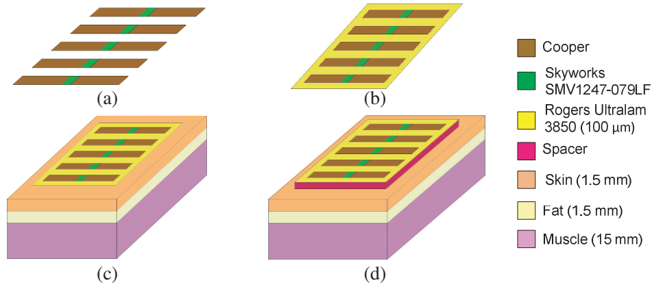
Figure 3. Structures simulated in HFSS: (a) dipoles in free space, (b) dipoles on substrate in free space, (c) FSS transponder placed on body model without spacer and (d) with different thickness of spacer.
