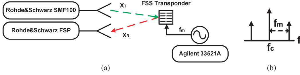
Figure 1. (a) Block diagram of the setup for experimental characterization. (b) Spectrum of the received signal.
