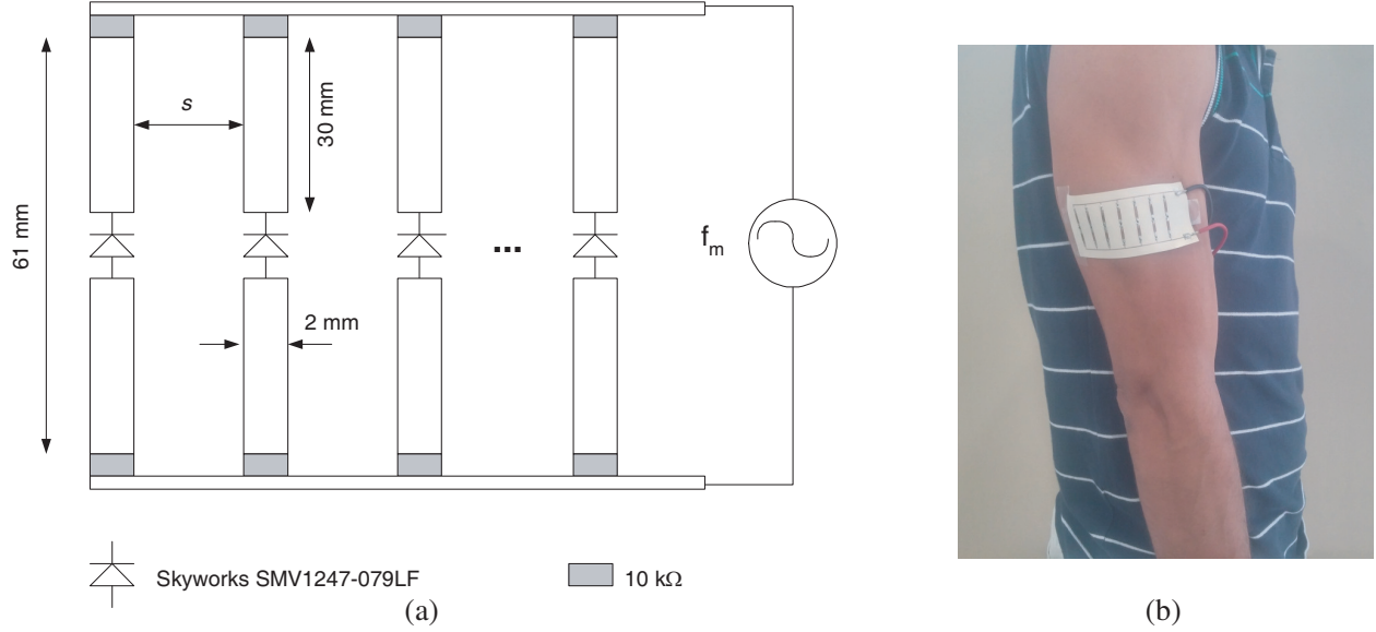
Figure 2. (a) FSS transponder basic schema used in the simulations and (b) prototype fabricated placed on the arm.
