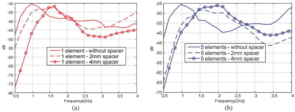
Figure 6. Comparison of FSS structure with (a) one and (b) five dipoles for different thickness of spacer between the FSS and the body.
